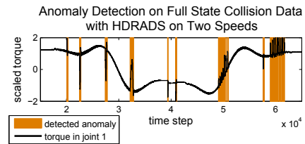
Fig. 7. Anomaly alarms from HDRADS during collision trajectory
